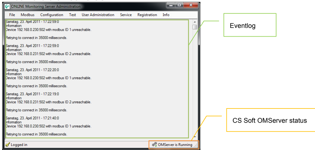
Illustration 20: Main Window
