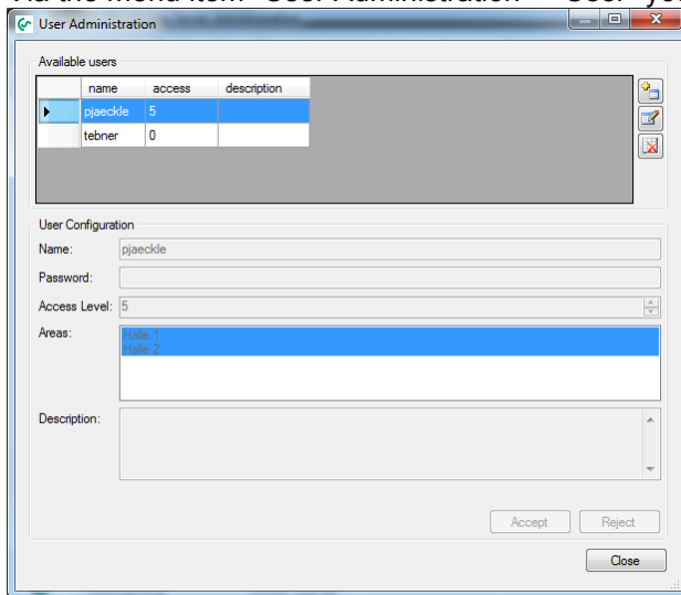
Illustration 19: User administration
