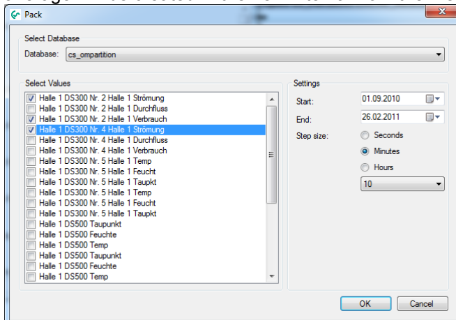
Illustration 25: Data Compression
