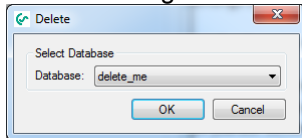
Illustration 27: Database deletion
